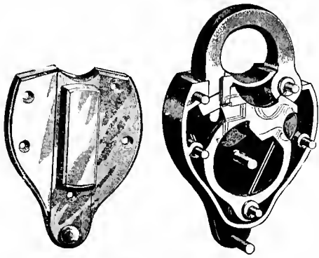
Figs. 2760-2761. RAILROAD PADLOCK, MALLEABLE IRON.
